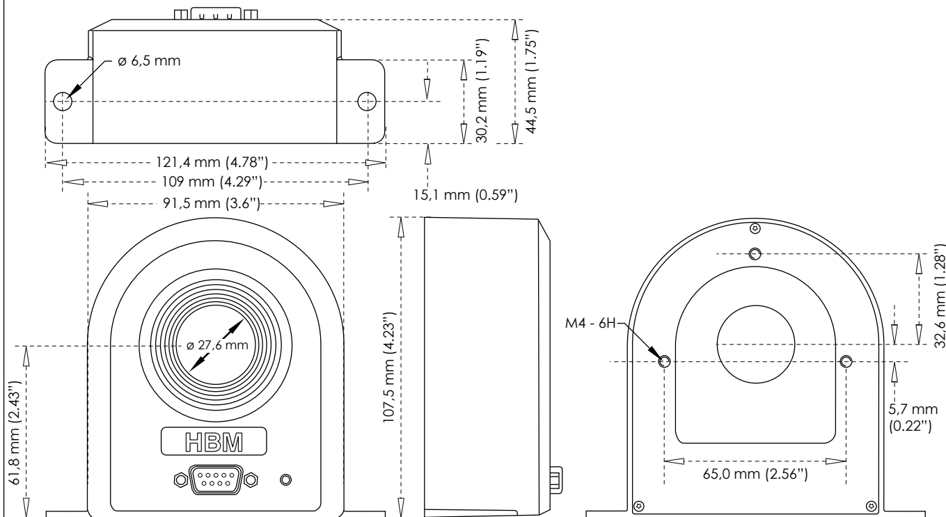
Figure 1.5 : Dimensions CTS50/200ID/400ID/600ID
