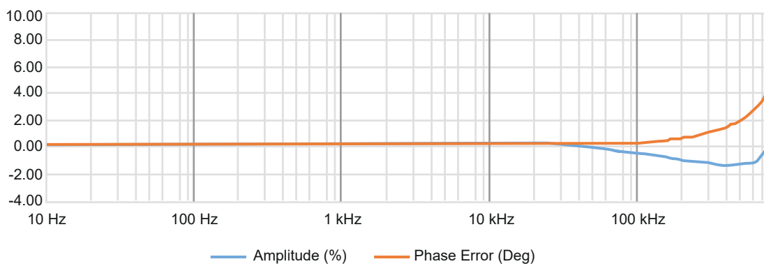
Figure 1.3: Frequency characteristics
