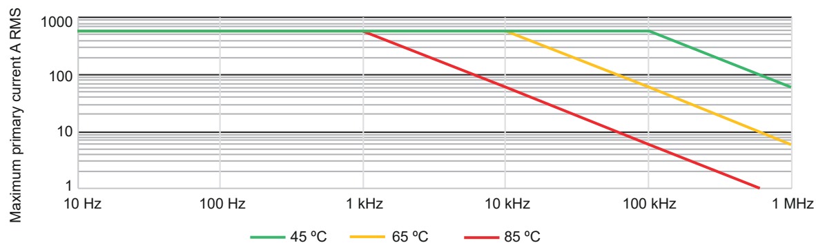
Figure 1.2: Frequency and ambient temperature derating
