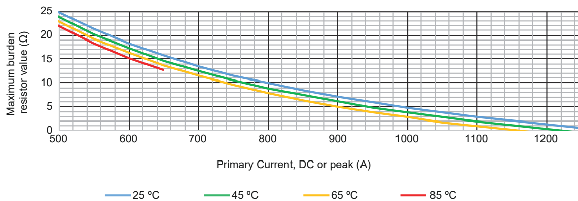
Figure 1.1: Burden resistor RM and ambient temperature derating
